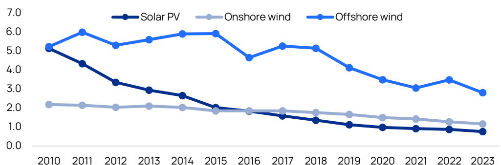
Figure 544: Global capacity-weighted average total installed cost of solar PV, onshore wind, and offshore wind power (USD mn/MW)
