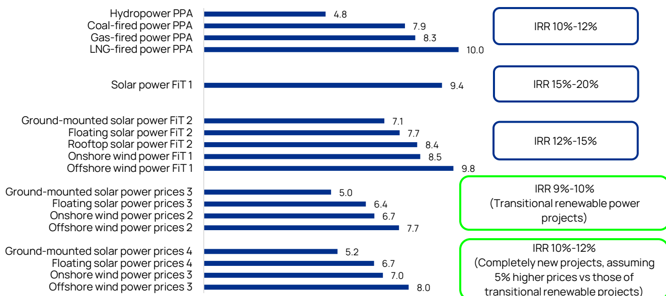
Figure 536: Contracted Power Purchase Agreement (PPA) prices of traditional power vs FiT and Vietcap's assumptions for new prices for renewable energy (US cents/kWh)
